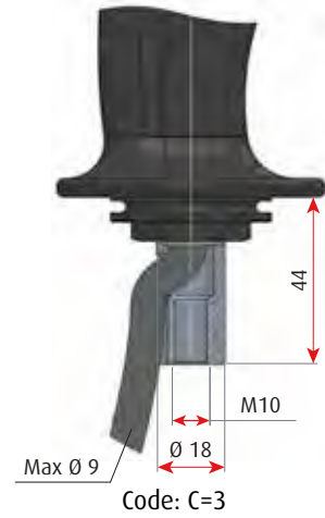
Connection with hole M10
