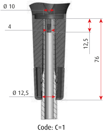
Joystick connection (2800 and 2900)
